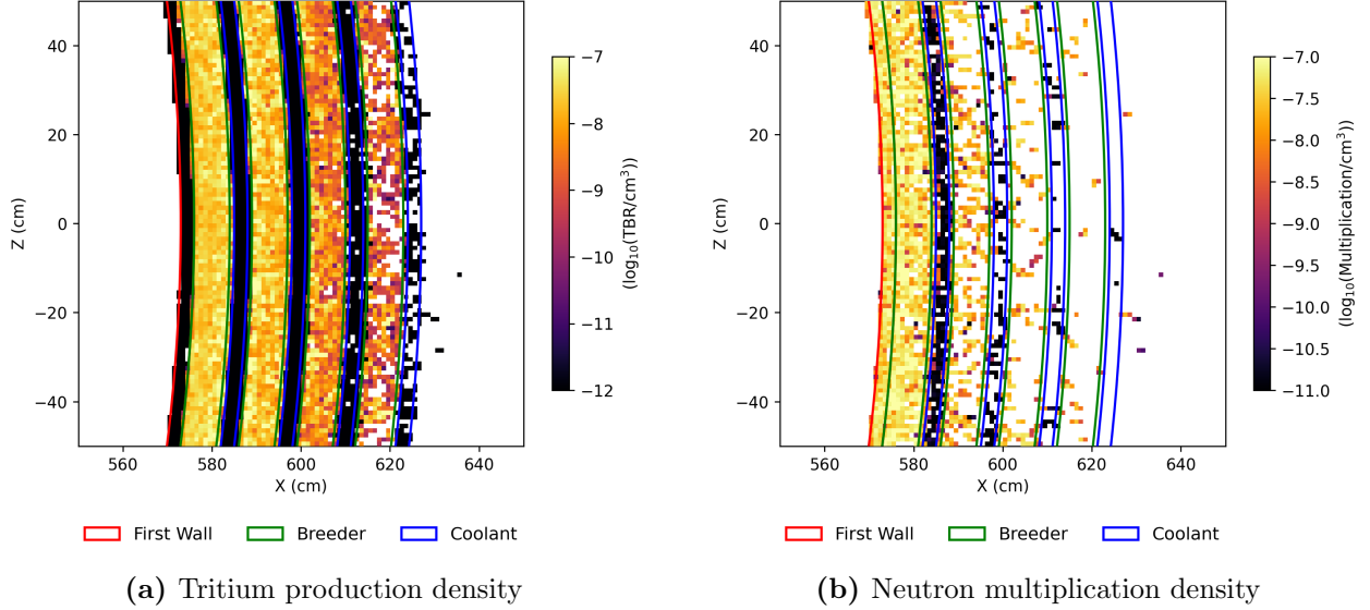
Figure 6: Cross-sectional heatmaps detailing the spatial distribution of key neutronic reactions. (a) Displays the density of tritium breeding reactions, strictly localised within the discrete breeder layers. (b) Illustrates the concentration of neutron multiplication events across the blanket depth. Trace reactions defined in Section 2.1.2 are also highlighted in the non-breeder layers, commonly shaded darker indicating rare events.
