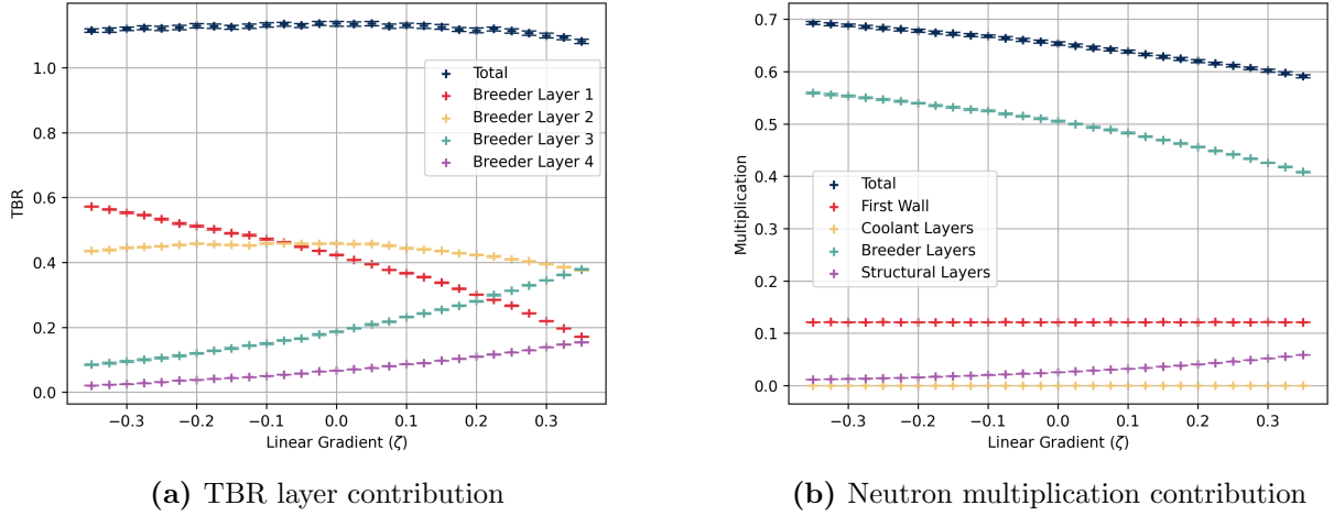
Figure 9: The impact of the linear gradient parameter ( \zeta ) on key neutronic performance metrics. (a) Tracks the total TBR and the individual contributions from discrete breeder layers. (b) Illustrates the total neutron multiplication alongside the specific contributions from the first wall, breeder, coolant, and structural separator layers. Statistical uncertainties are plotted, though error bars are generally smaller than the data markers.
