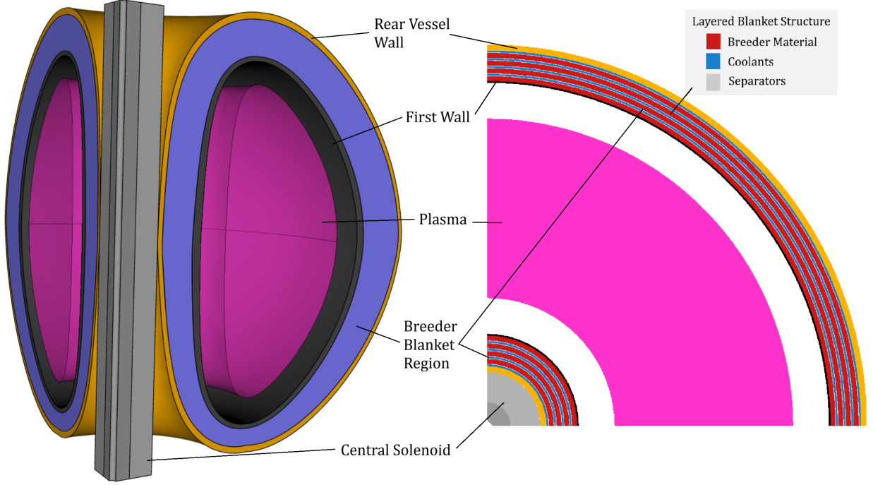
Figure 1: Representative geometry of the simplified Tokamak model generated via Paramak. The simulation domain comprises a 90° revolution with periodic boundary conditions. Included is an example breakdown of the layered blanket, only the coolant and breeder thicknesses are adjusted in this study.
